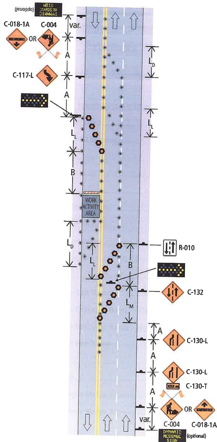
Figure 8.14: Passing/Climbing Lanes – Lane Shift – Short and Long Duration
